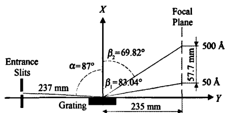
图 2 平场极紫外光谱仪光路示意图 Fig.2 Flat-field EUV grating spectrograph's principle.
