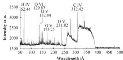
图 5 EAST 装置等离子体 50–500 Å 谱线 Fig.5 Spectral region of 50–500 Å in EAST tokamak plasma.
