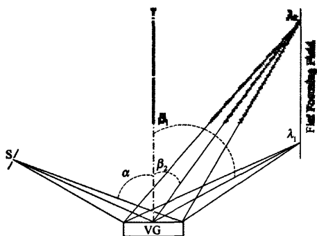
图 1 凹面等间距光栅(a)和凹面变线距光栅(b) Fig.1 Concave grating with invariable line space (a) and variable line space (b).
