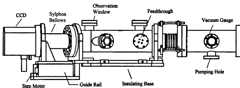
图 3 EUV 光谱仪结构示意图 Fig.3 Outside diagram of EUV spectrometer.
